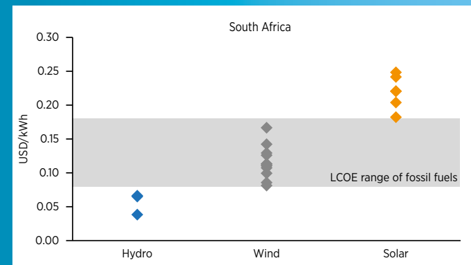
Figure 3: Levelised costs of electricity generation for selected grid-connected projects in South Africa and East Africa
