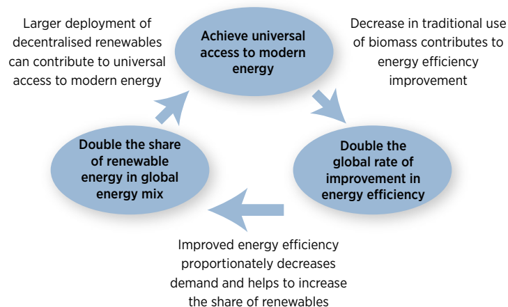
Figure 7: Virtuous cycle of SE4ALL goals
