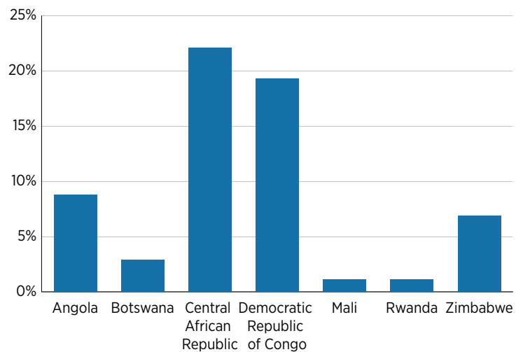
Figure 5: Losses due to electrical outages as percentage of annual sales (2010 and 2011 data)
