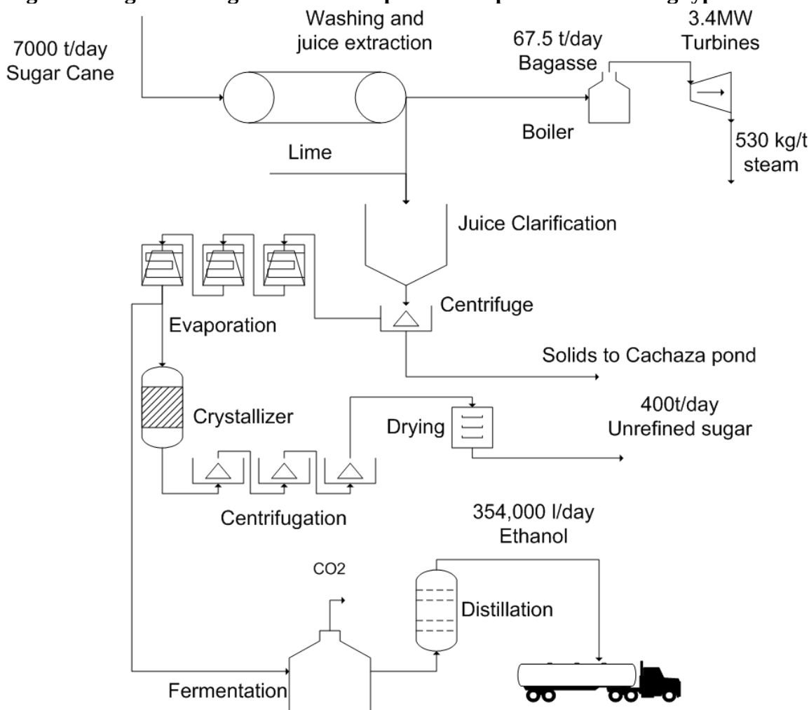
Figure 2: Sugarcane sugar and ethanol production process illustrating typical mill
