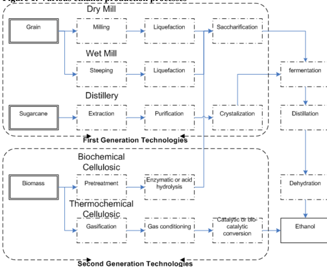
Figure 1: Various ethanol production processes
