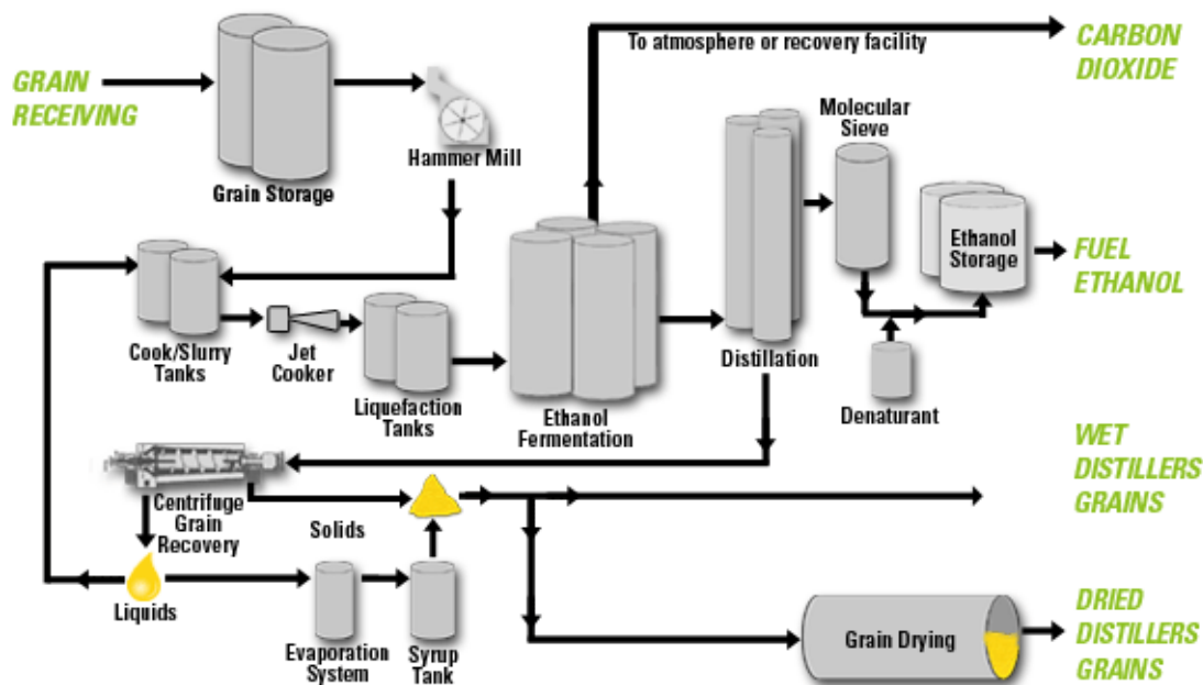
Figure 6: Dry Grind Ethanol Production Process
