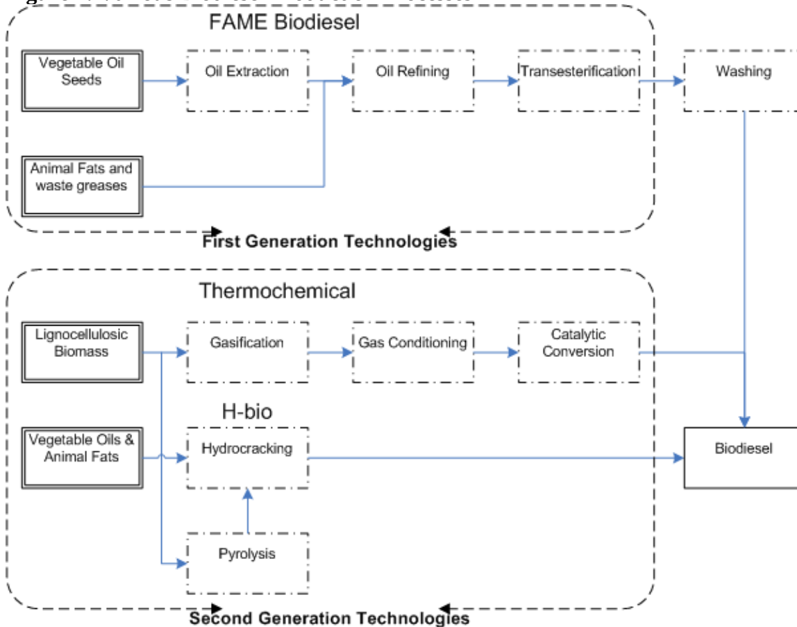
Figure 7: Various Biodiesel Production Processes
