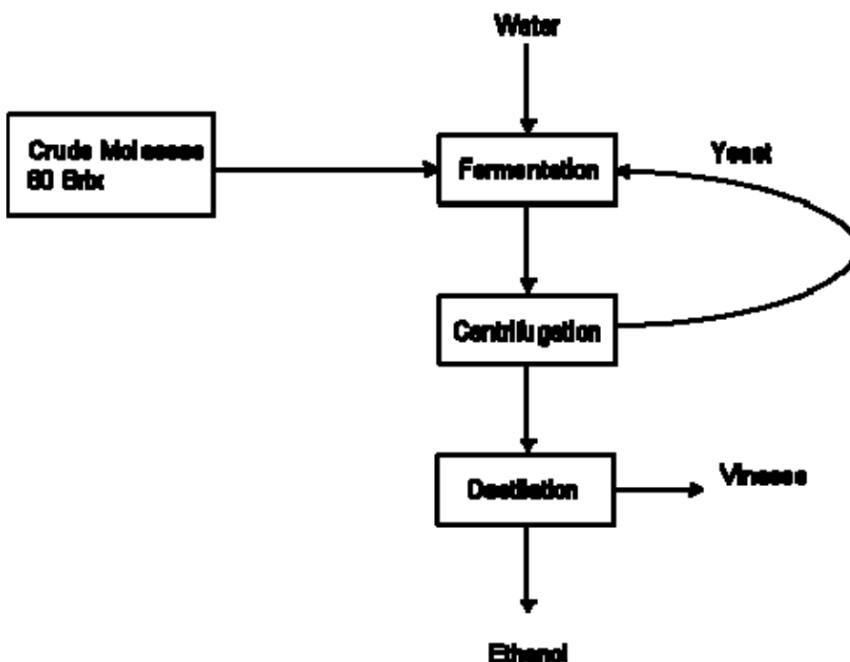
Figure 3: Ethanol production process based on molasses
