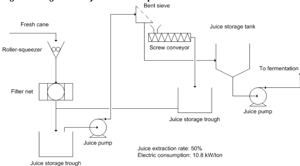
Figure 5: Sorghum cane juice extraction process
