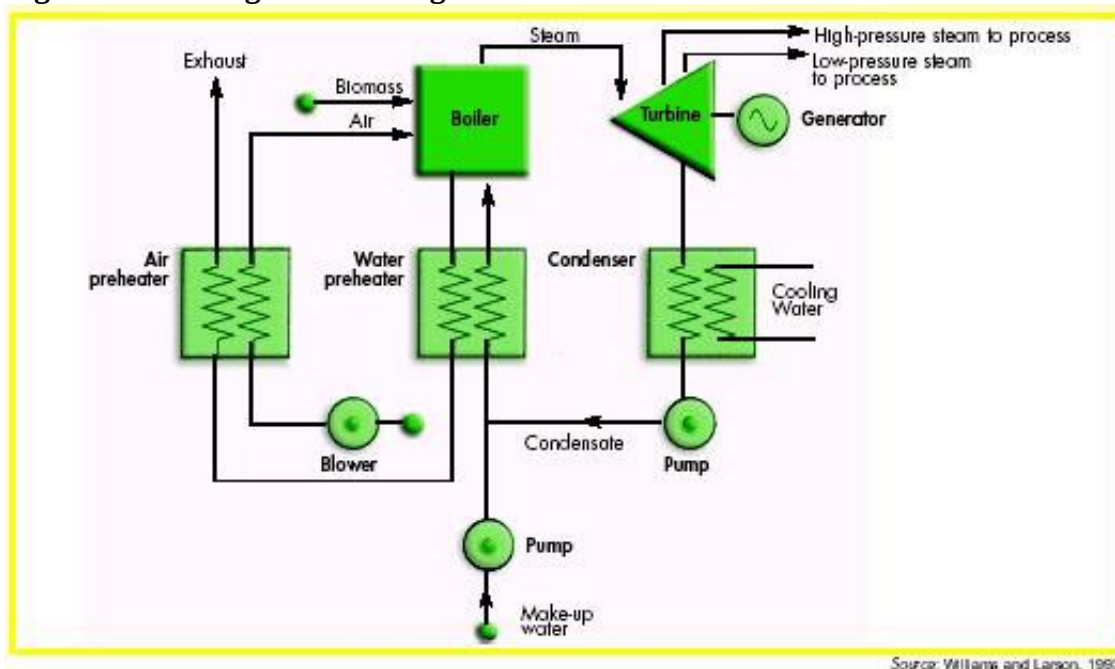
Figure 15: Schematic diagram of a biomass-fired steam-Rankine cycle for cogeneration using a condensing-extraction steam turbine
