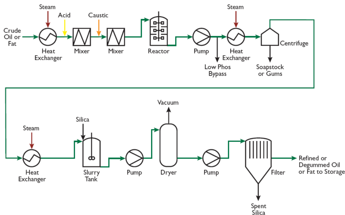
Figure 10: Vegetable Oil and fat Refining (Pre-treatment)
