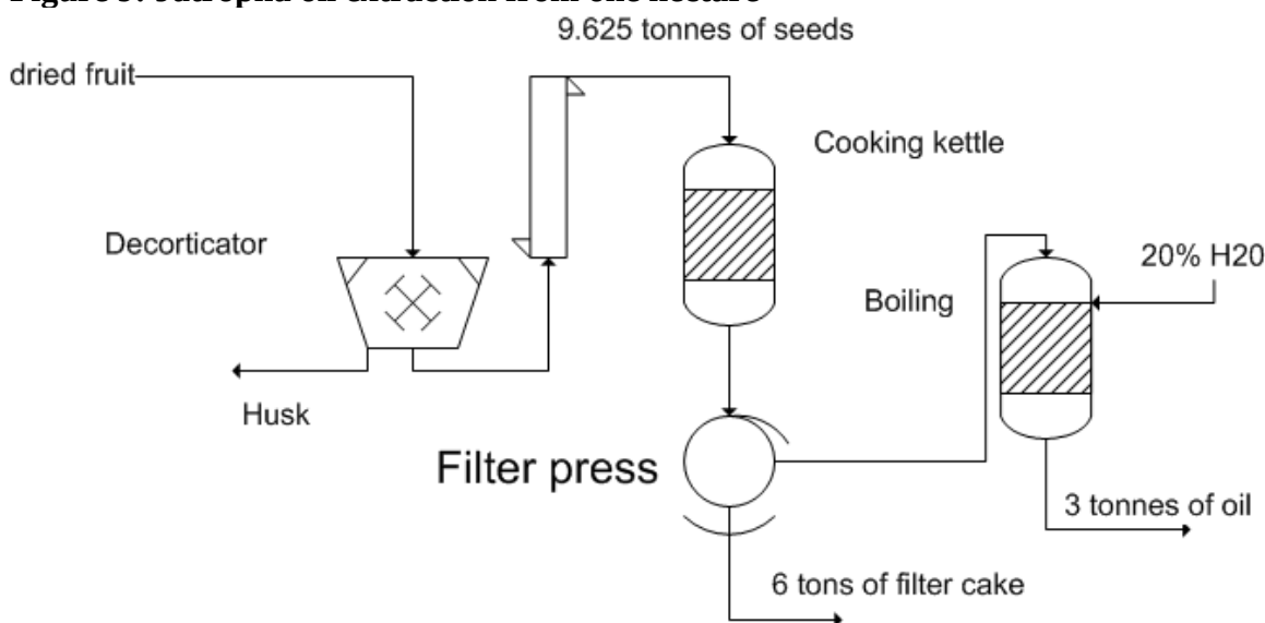
Figure 9: Jatropha oil extraction from one hectare
