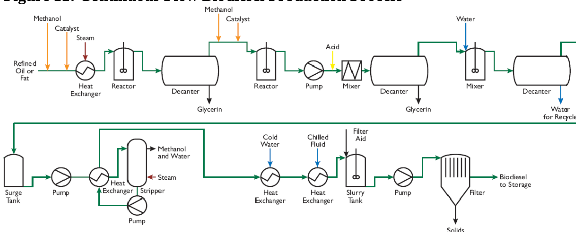
Figure 11: Continuous Flow Biodiesel Production Process
