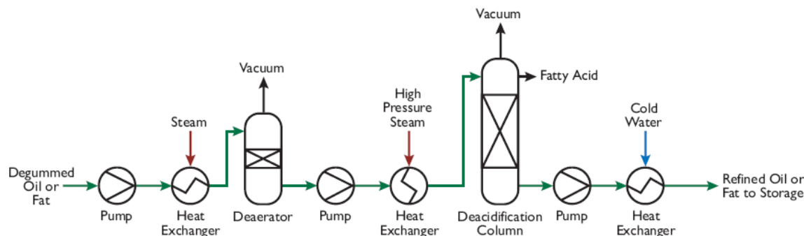
Figure 12: High FFA oil pre-processing
