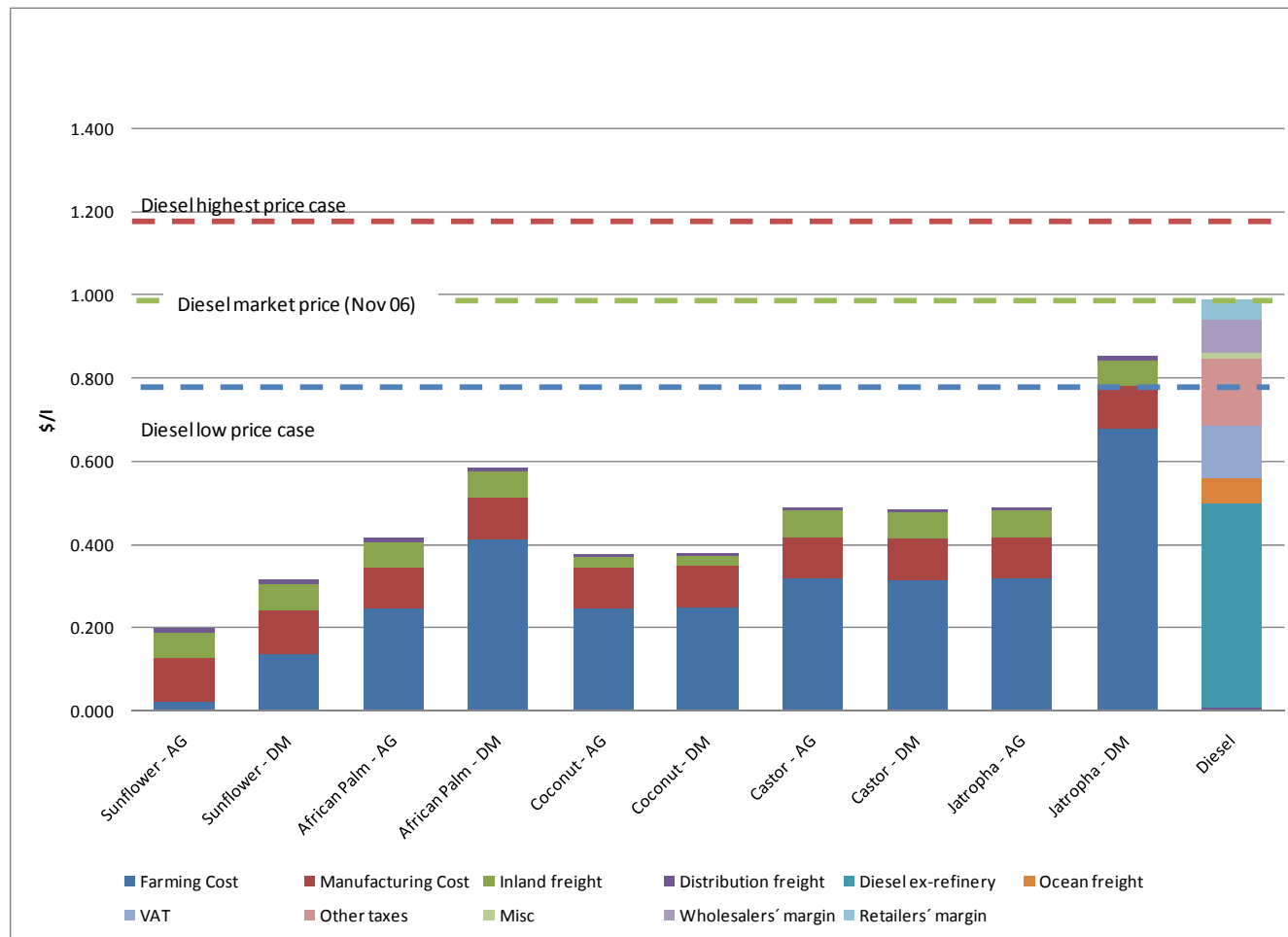
Figure 5: Comparison of biodiesel based on different raw materials and costs with the sale price of diesel at the pump, with large-scale production units
