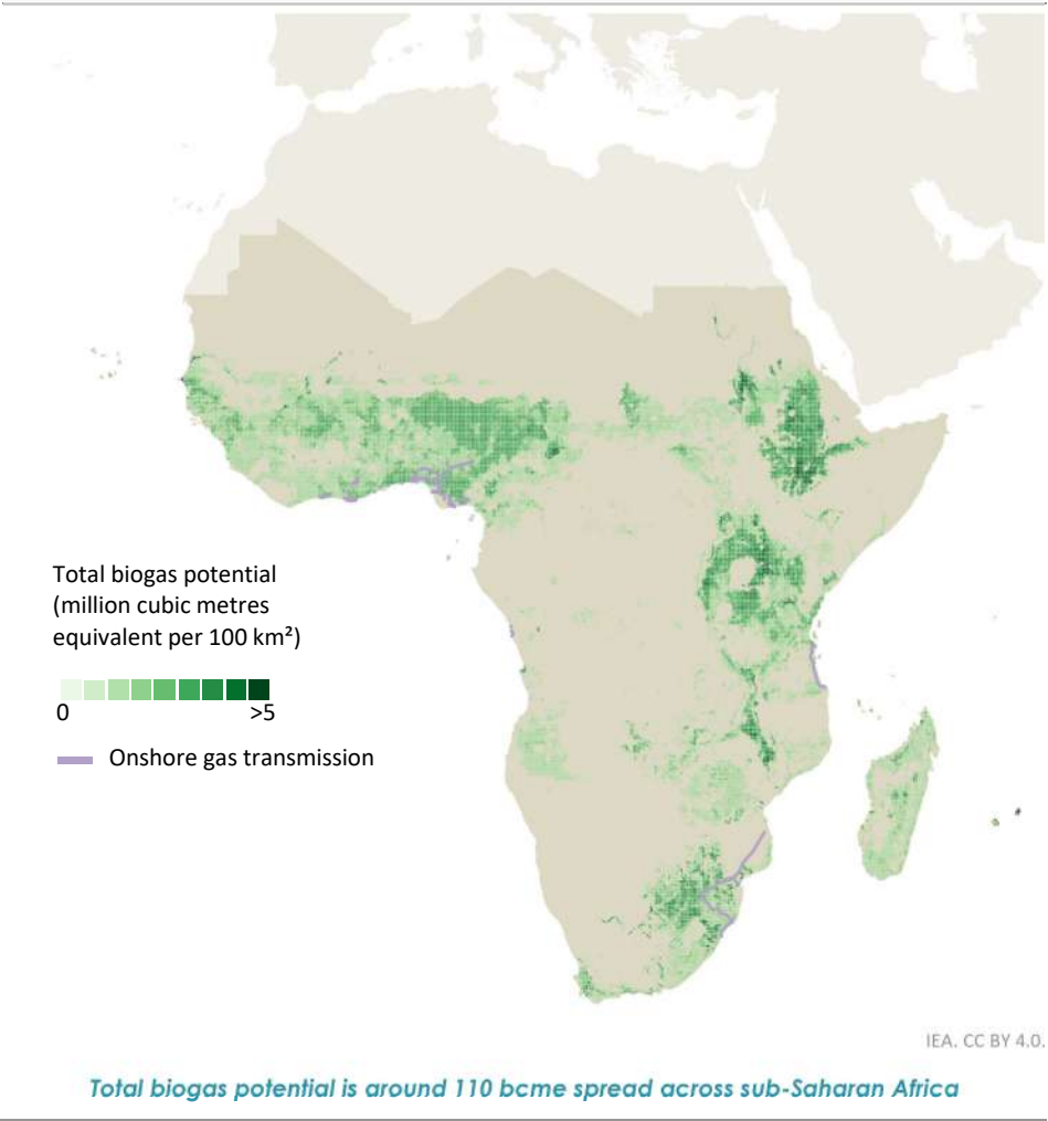
Figure 3.11 ▶ Biogas potential in sub-Saharan Africa, 2024
