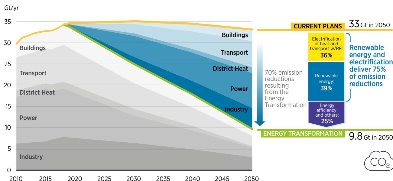
Figure 1.1: Annual energy-related CO 2 emissions and reductions, 2010–2050
