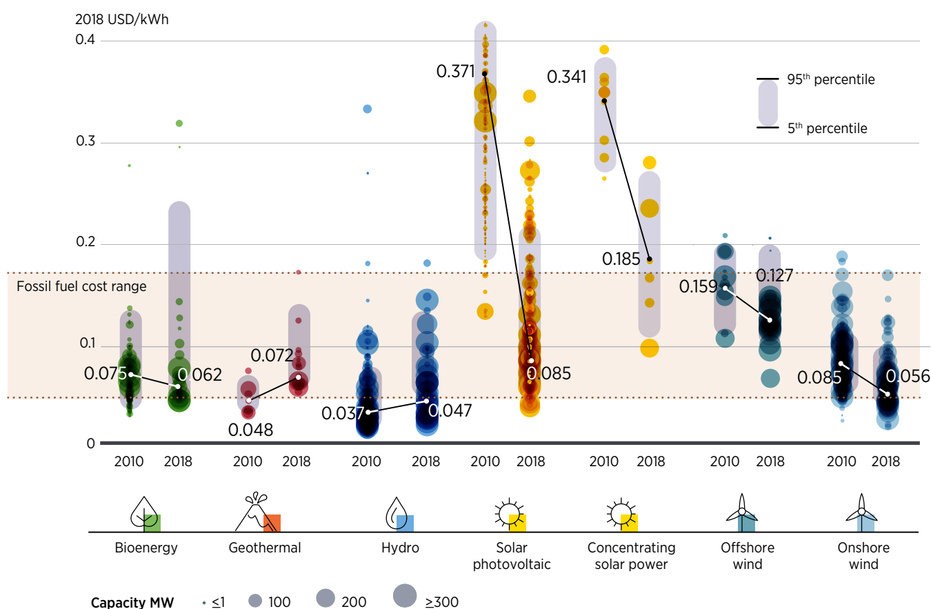
Figure 1.4: Global electricity costs from utility-scale renewable power generation, 2010–2018
