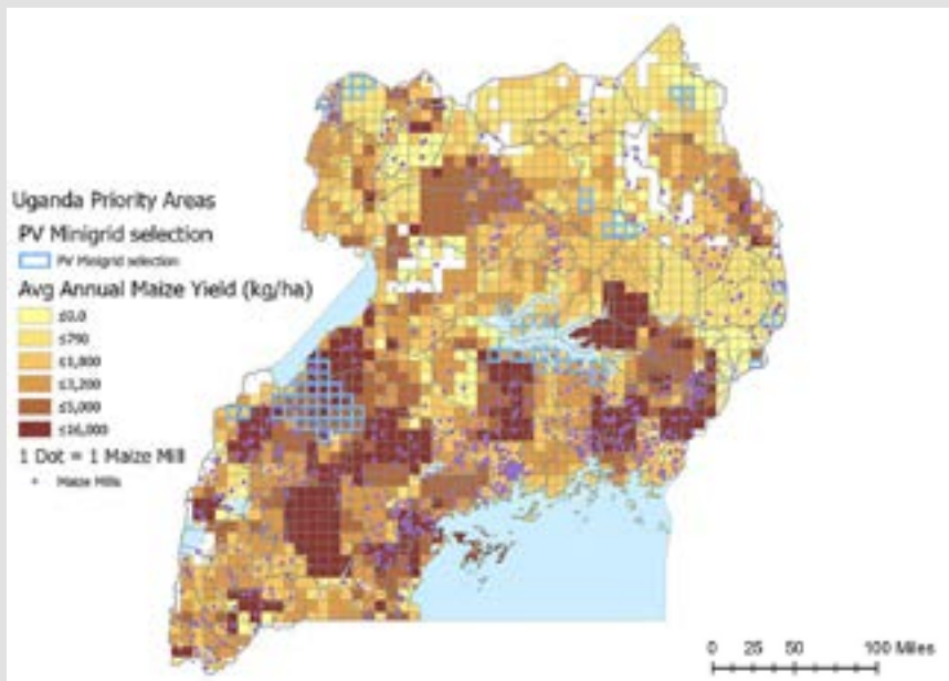
FIGURE 4.6 Priority areas for linking mini-grid supply with maize processing
