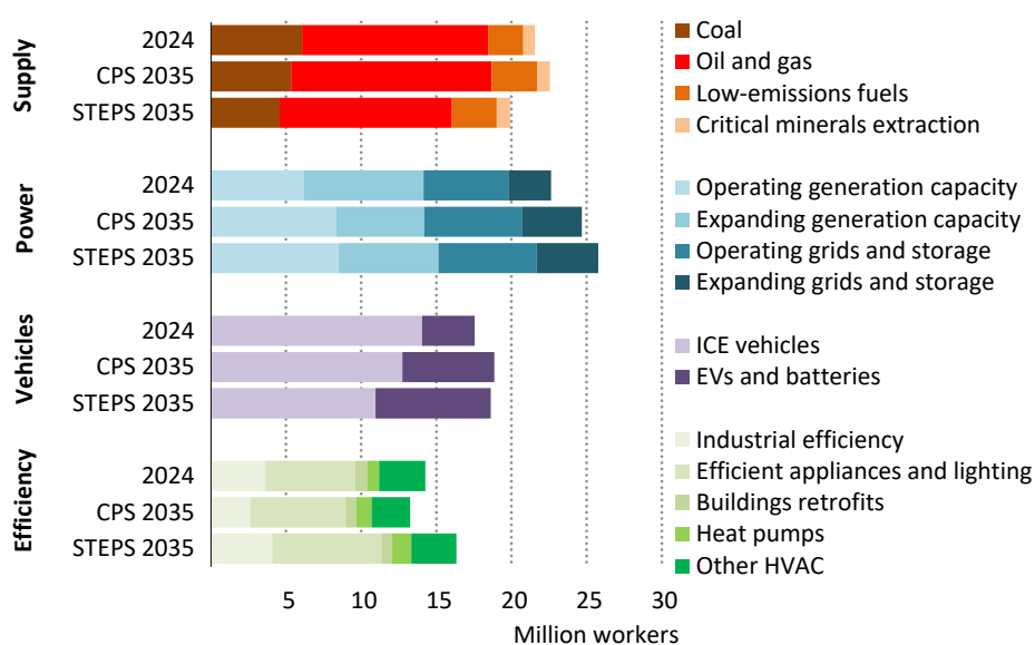
Figure 5.39 ▶ Global energy-related employment by type and scenario, 2024 and 2035
