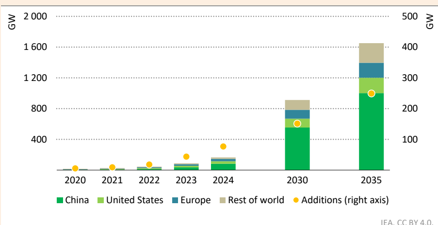
Figure 5.13 ▶ Global installed battery storage capacity and additions, 2020–2024, and in the STEPS, 2030 and 2035
