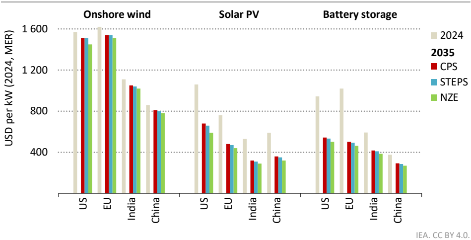
Figure 2.14 ▶ Installed costs of onshore wind, solar PV and battery storage by scenario and region/country, 2024 and 2035
