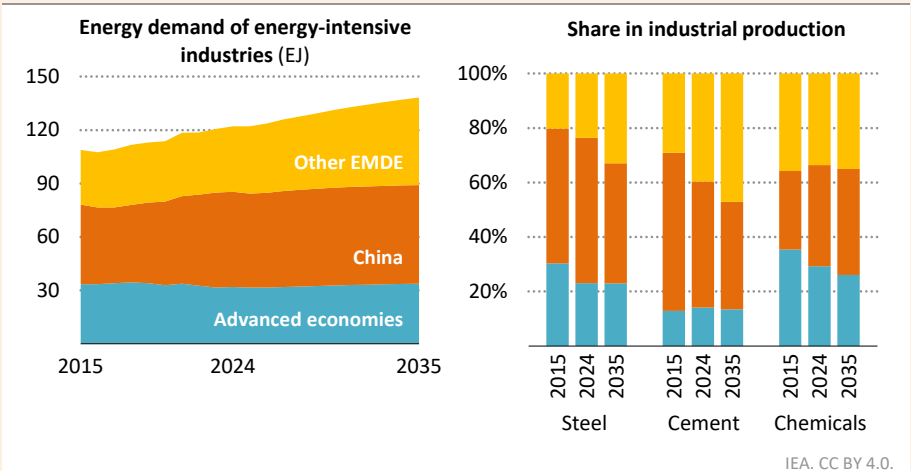
Figure 3.14 ▶ Energy demand of energy-intensive industries, and industrial production in selected sub-sectors in the CPS to 2035
