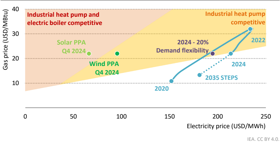
Figure 8.15 ▶ Competitiveness of electrification routes compared to average end-user prices for industrial consumers in the Europe Union
