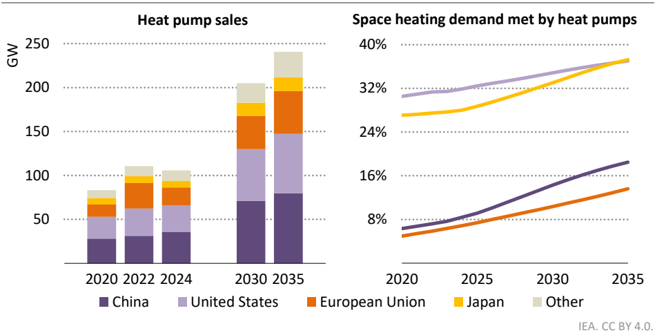
Figure 4.11 ▶ Global heat pump sales and contribution to space heating demand in selected regions in the STEPS, 2020-2035
