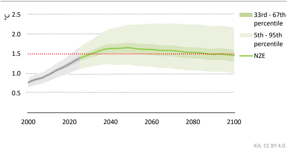
Figure 7.10 ▶ Temperature rise in the NZE Scenario, 2000-2100
