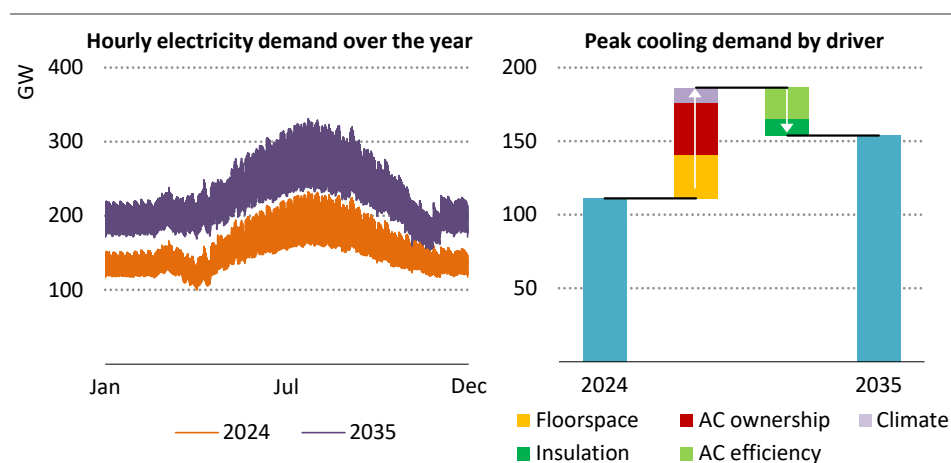
Figure 8.21 ▶ Annual electricity load curve and peak cooling demand by driver in the Middle East in the STEPS, 2024-2035
